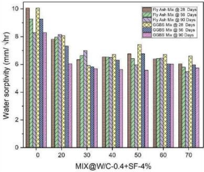
Figure 10 Water Sorptivity with W/C ratio 0.4 with FA and GGBS with 4% SF.
