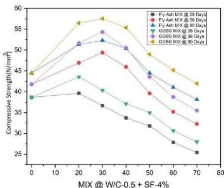
Figure 6 Results of ternary blend of cement concrete fixing 4% SF with 0.5 W/B ratio of both FA and GGBS.
